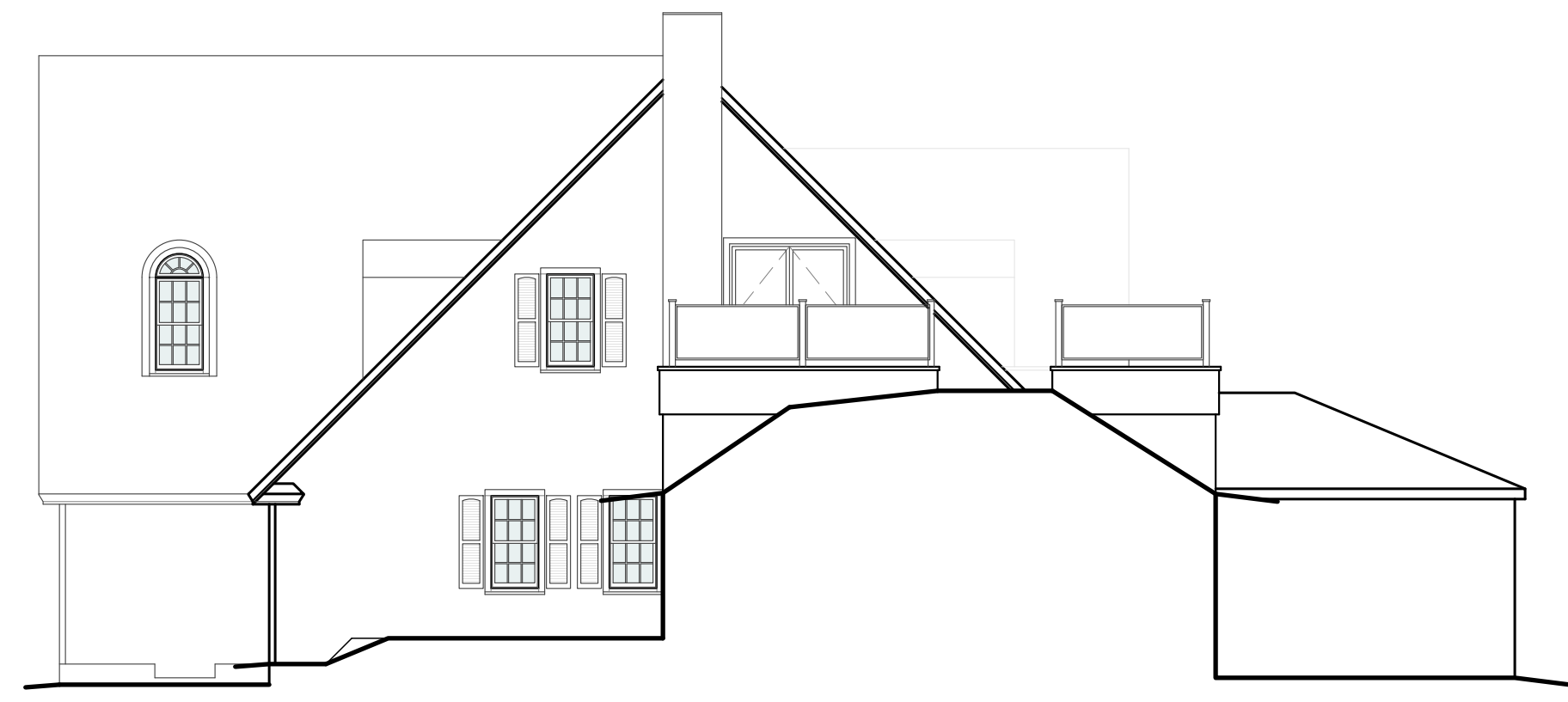
SOUTH ELEVATION 1/8" = 1'-0"
