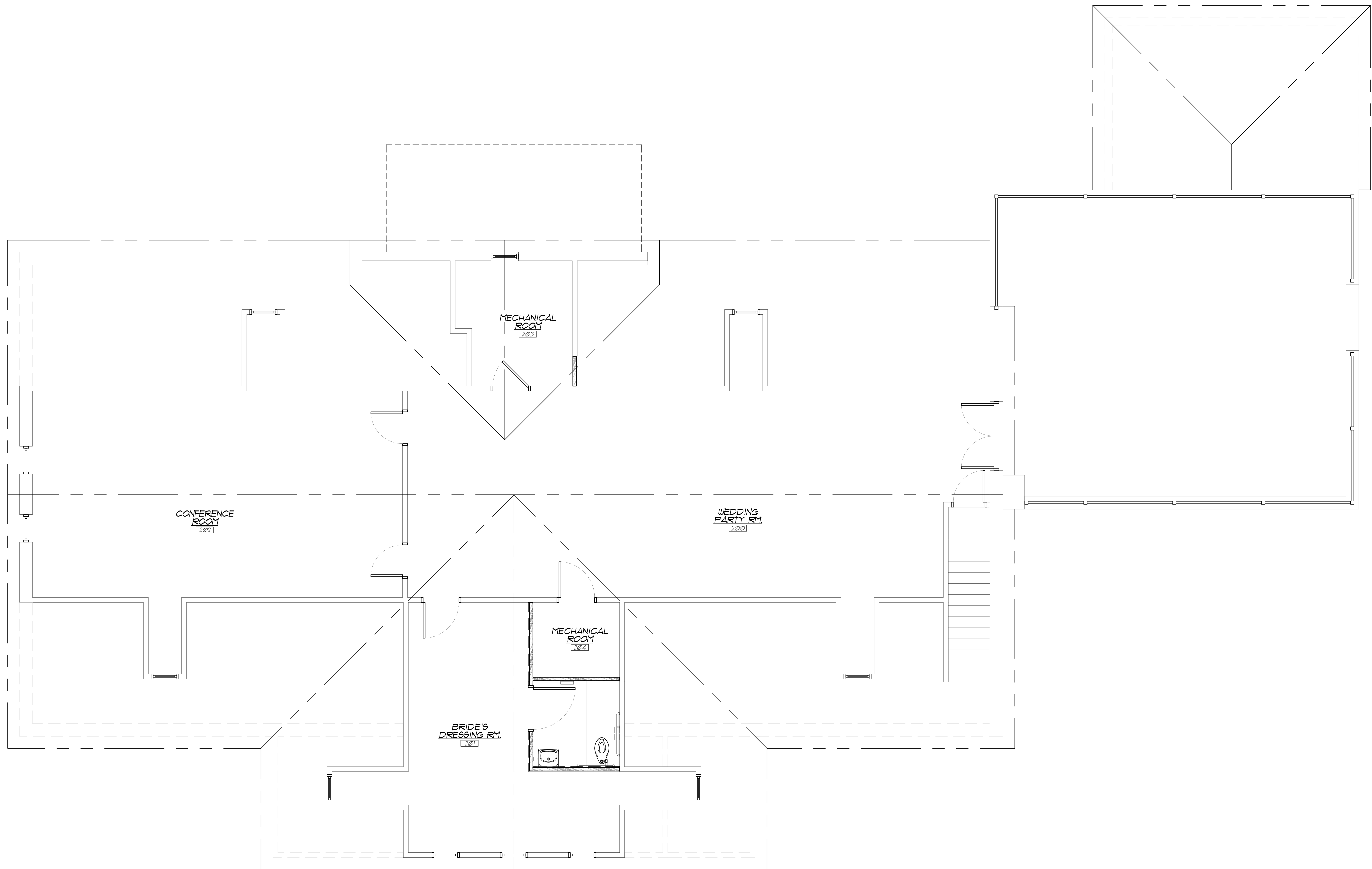
SECOND FLOOR PLAN SCALE 1/4" = 1'-0" NORTH
