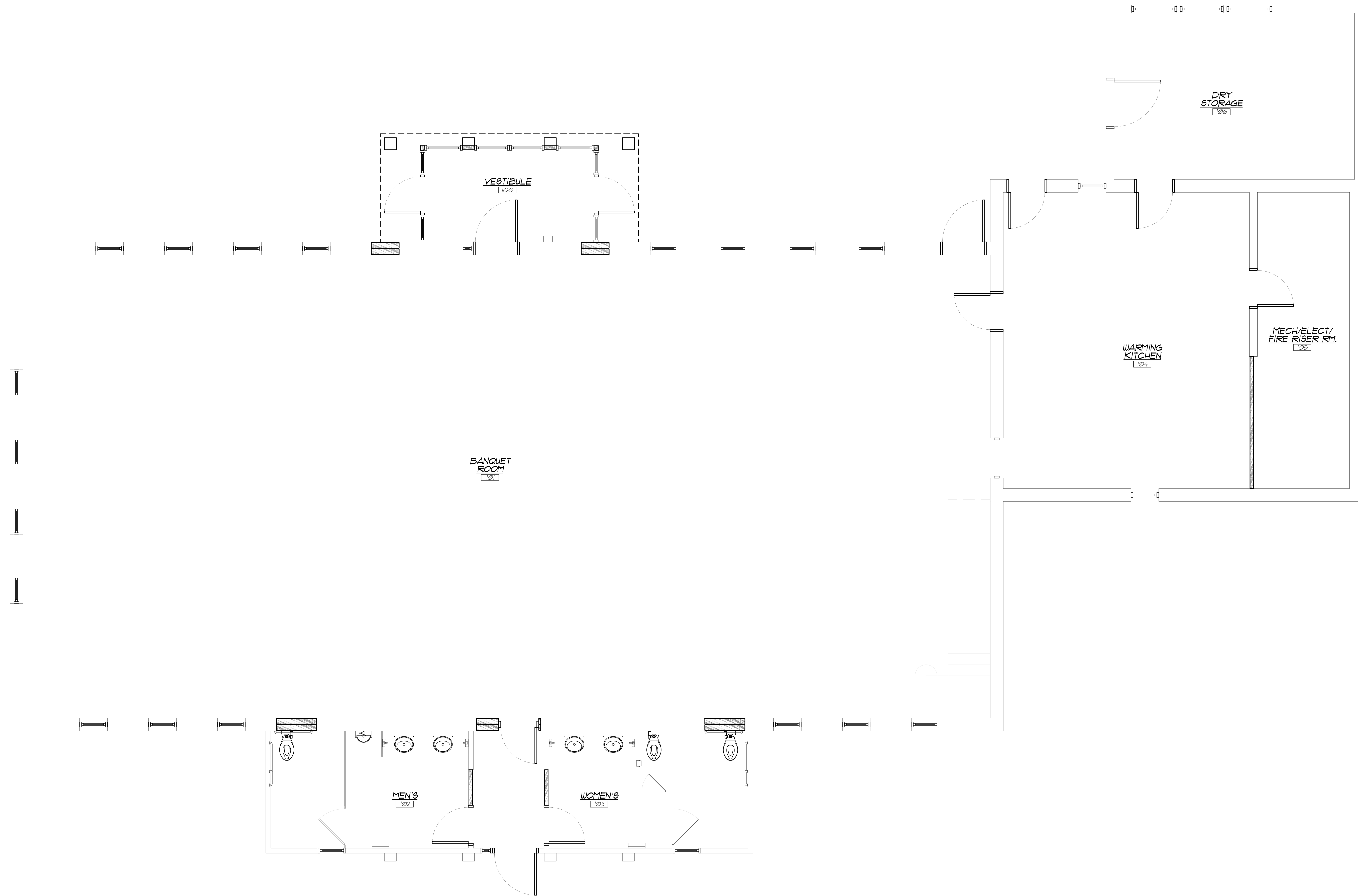
FIRST FLOOR PLAN SCALE 1/4" = 1'-0" NORTH
